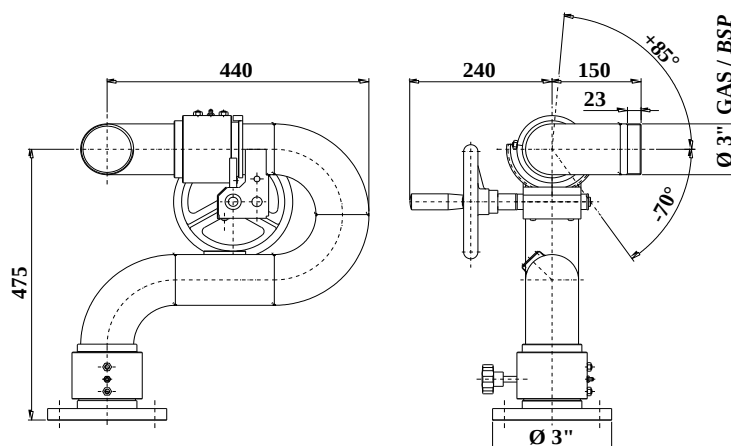
Mod. SE-KM-V-3X 1 volante/1 handwheel
