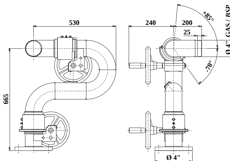
Mod. SE-KM-2V-4X 2 volantes/2 handwheel
